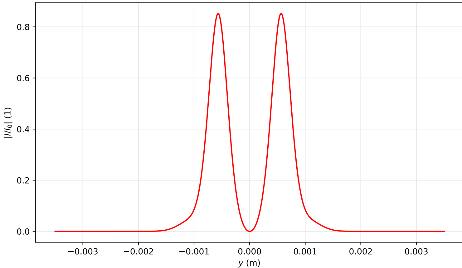
Intensity profile I(x=0, y, z=0.796)/I_0 , P_{in}=4.0P_{cr} , artificial time
